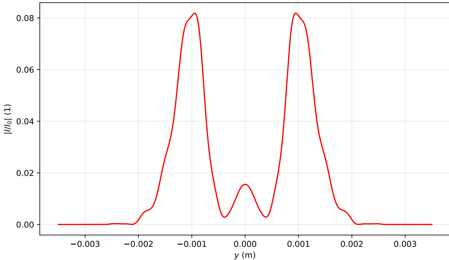
Intensity profile I(x=0, y, z=3.105)/I_0 , P_{in}=7.5P_{cr} , artificial time
